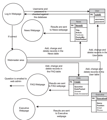
Data Flow Diagram for SQL Database
